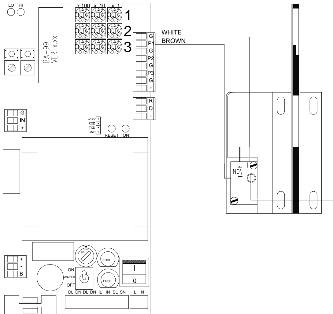
Figure 21:Wiring of Range Servant Token Control.
