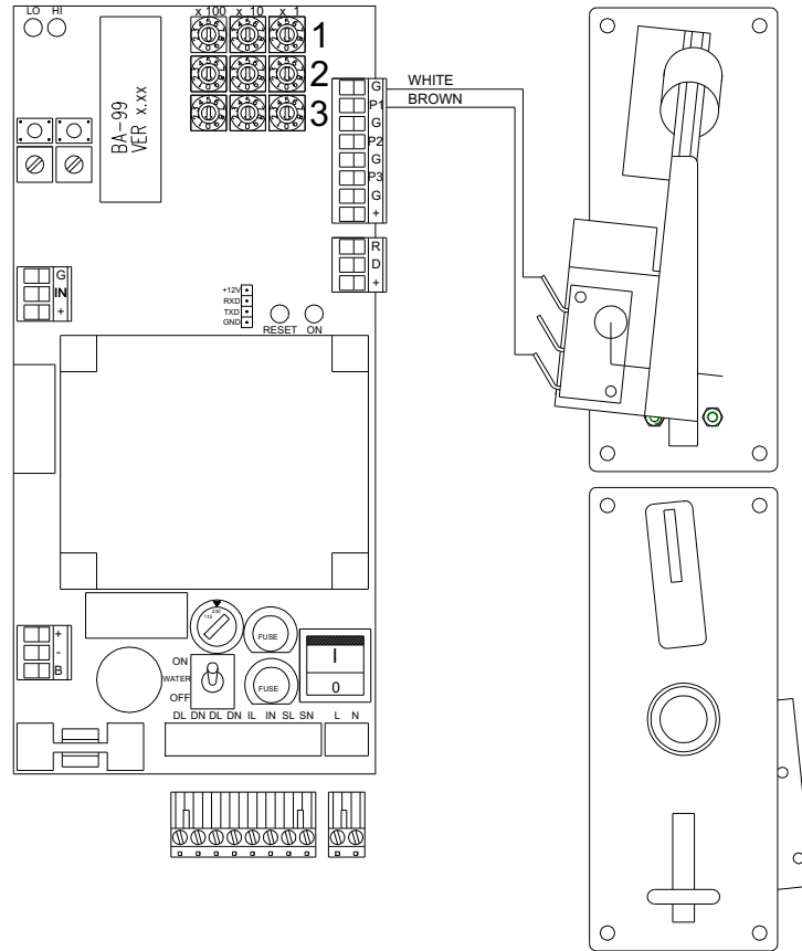
Figure 19: Wiring of the mechanical coin control
