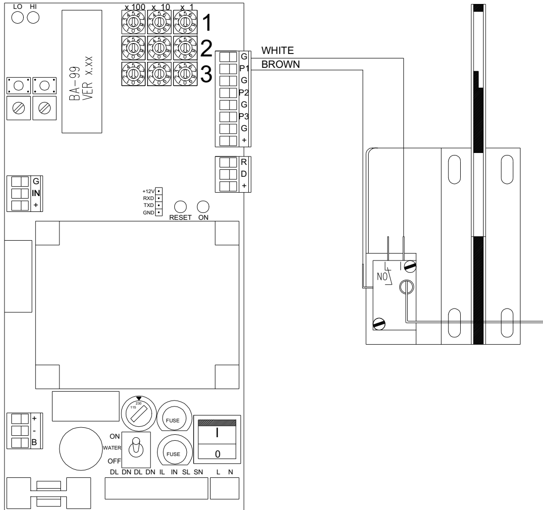
Figure 18: Wiring of the Range Servant Token Control.
