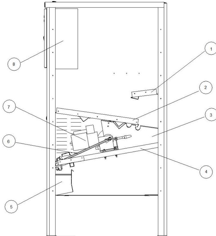
Fig. 7: Inside of the ball dispenser, side view
