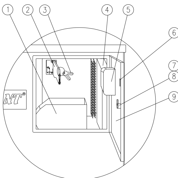
Fig. 20: Control box
