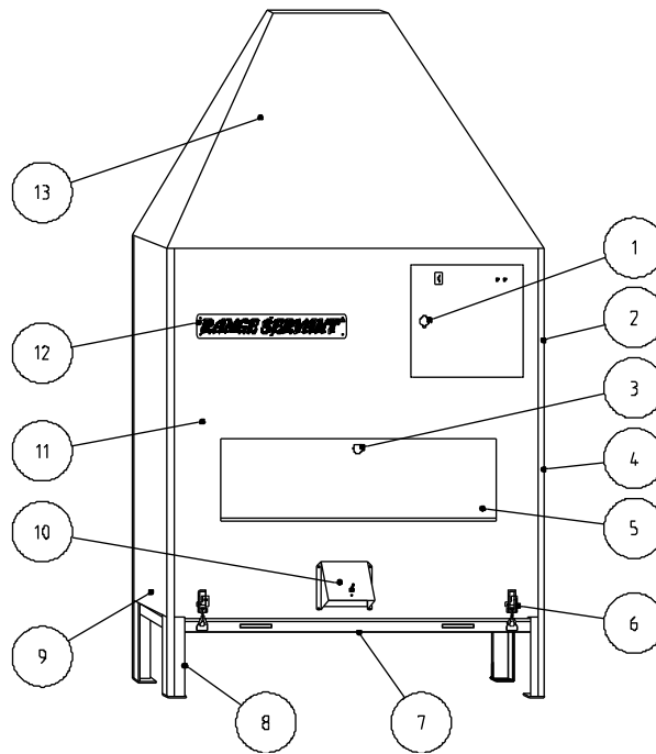
Figure 34: External RS-18
