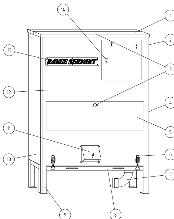
Figure 34: Extérieur RS-8
