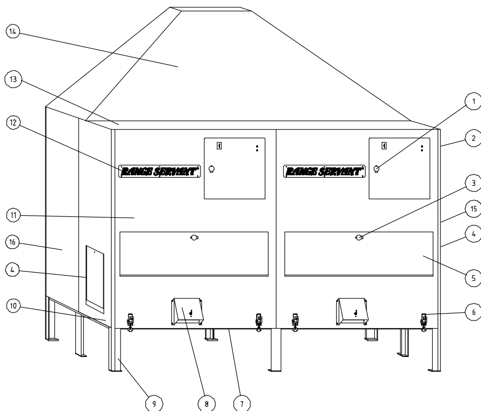
Figure 37: Extérieur RS-45
