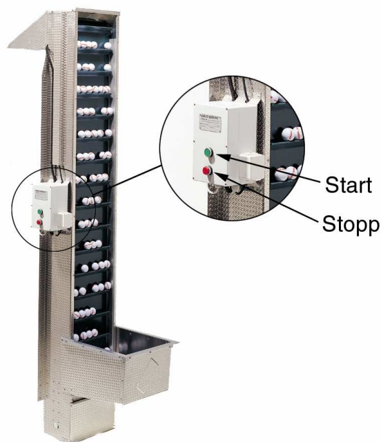
Figure 4: Location of the Start/Stop switch
