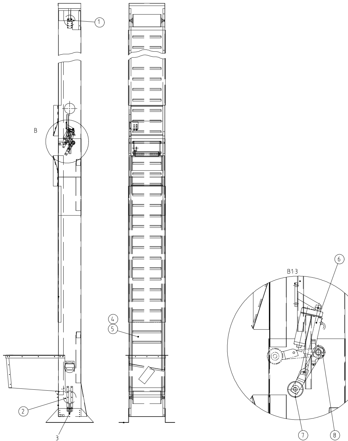
Figure 15: Multi-storey elevator
