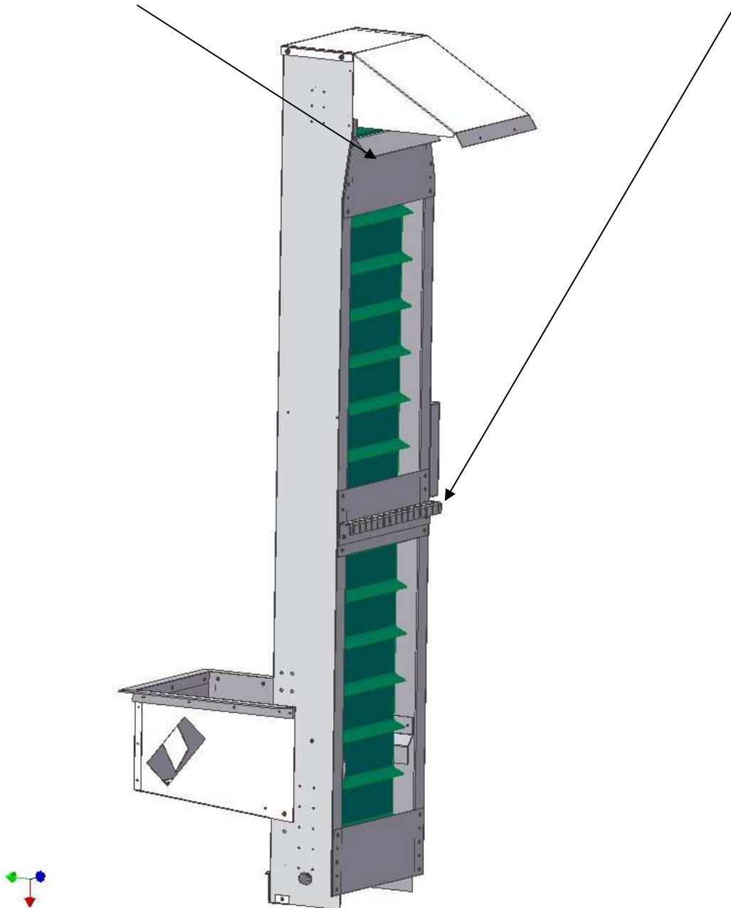
Figure 13: Elevator for BTW dispensers
