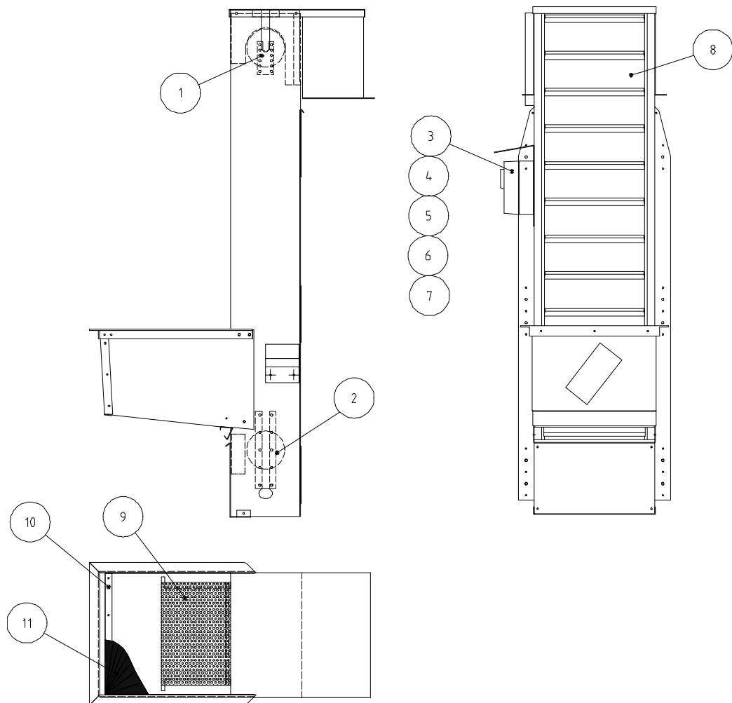
Figure 11: Elevator for machines with a flat top
