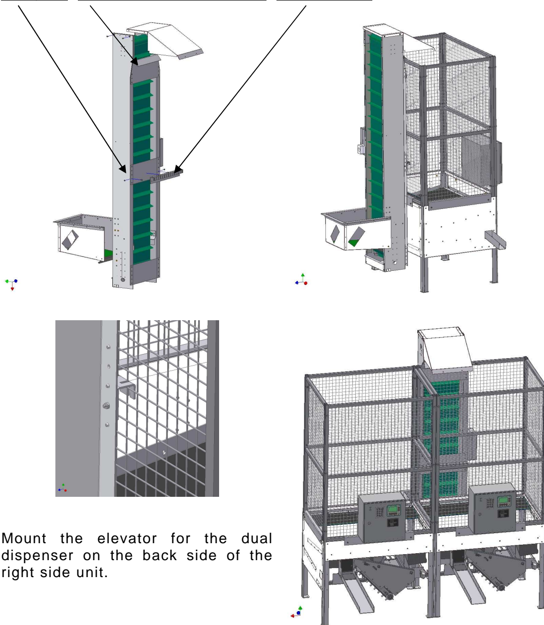
Figure 10: Mounting the elevator for BTW dispense
