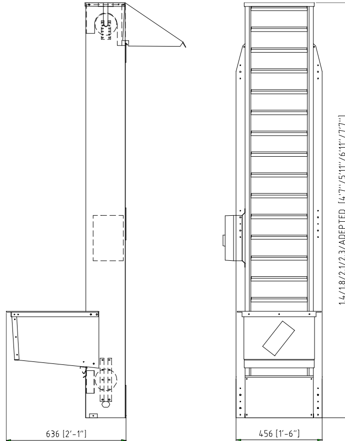
Figure 2: Main measurements
