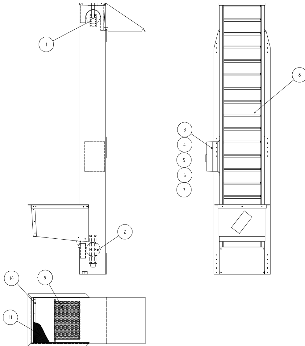
Figure 12: Elevator for machines with a conic top
