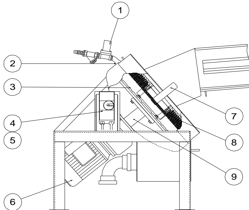
Figure 12: Ball Washer BT 1950, side view
