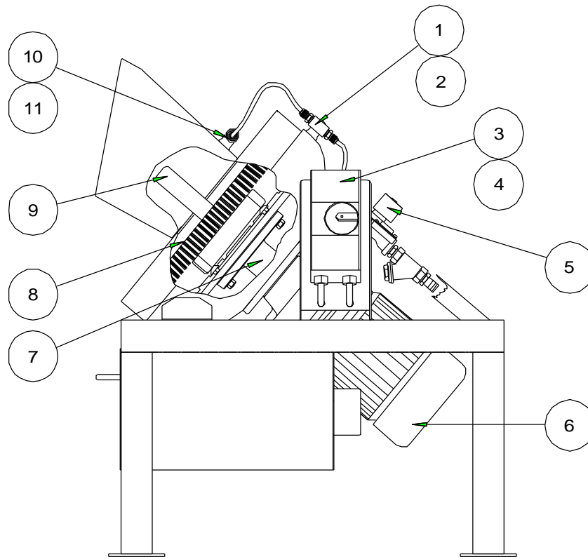
Figure 13: Ball Washer BT 1300, side view
