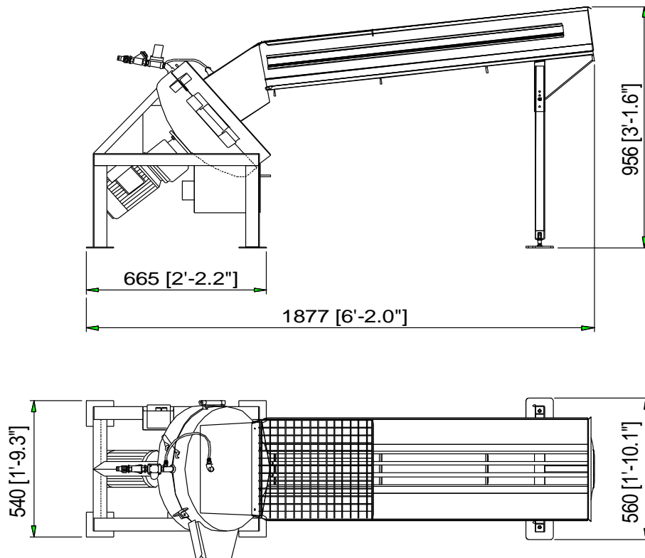
Figure 2: Ball Washer BT1950
