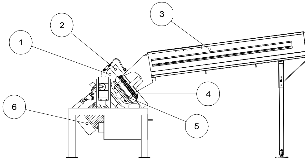
Figure 6: Ball Washer, side view
